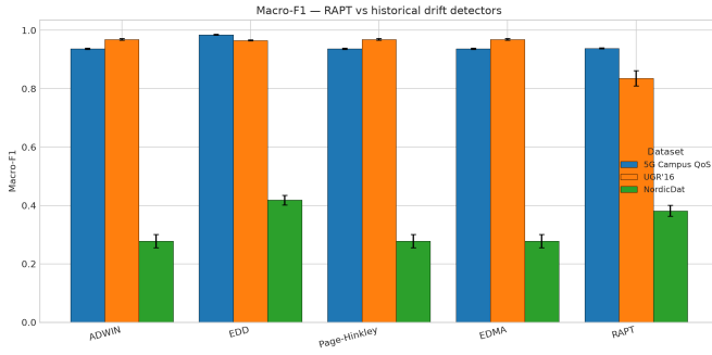
Fig. 6. Historical detectors. ADWIN, Page-Hinkley and EDMA never fire, so they replicate the frozen baseline. EDD fires most often, reaching the highest macro-F1 at the highest adaptation cost. RAPT adapts less often than all but two methods, and less accurately.
