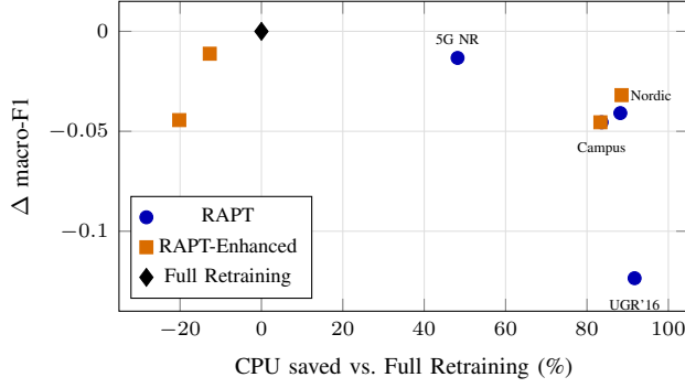
Fig. 4. Accuracy–cost trade-off on all four streams, measured against Full Retraining at the origin. Circles are RAPT and squares are RAPT-Enhanced, computed from Table II. Up and to the right is better. Squares left of zero cost more adaptation CPU than Full Retraining.
